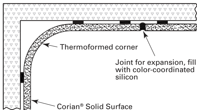
FIGURE H-1: ADJACENT SILICONE SOFT SEAMS
