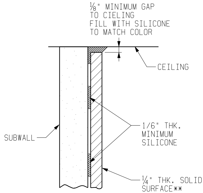
WALL HEAD DETAIL
